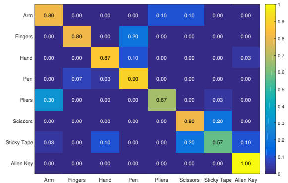
Fig. 4: Confusion matrix of the SURF-based method.
